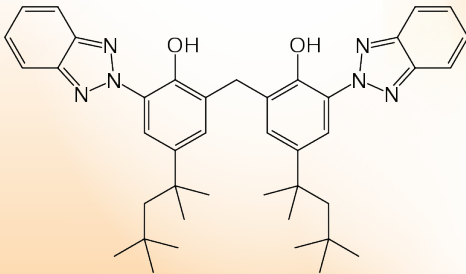
The molecular structure of Tinosorb M
