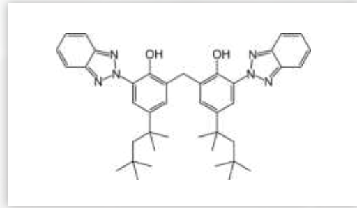
THE MOLECULAR STRUCTURE OF TINOSORB M
